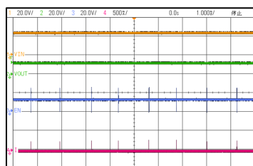
图 5.2-5 Steady State Power Save Mode
