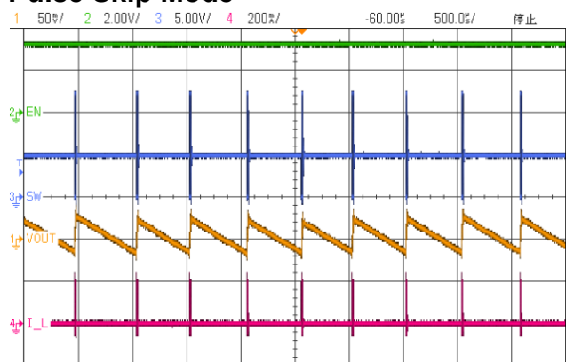
Figure 10.e V_{IN}=5\text{V} , V_{OUT(AC)}=12\text{V} , LOAD=1mA L=10\mu\text{H} , C_{OUT}=10\mu\text{F} , C_{IN}=4.7\mu\text{F}
