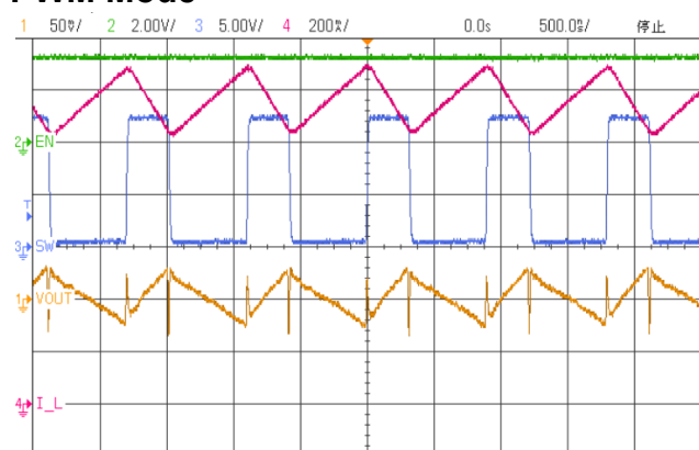
Figure 10.c V_{IN}=5\text{V} , V_{OUT(AC)}=12\text{V} , LOAD=400mA L=10\mu\text{H} , C_{OUT}=10\mu\text{F} , C_{IN}=4.7\mu\text{F}
