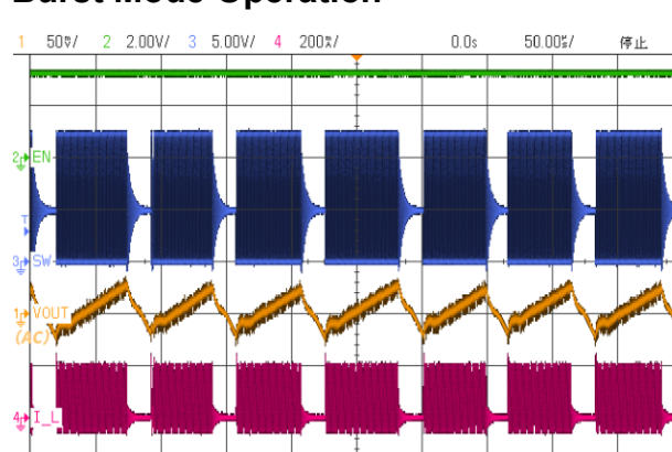
Figure 10.d V_{IN}=5\text{V} , V_{OUT(AC)}=12\text{V} , LOAD=20mA L=10\mu\text{H} , C_{OUT}=10\mu\text{F} , C_{IN}=4.7\mu\text{F}
