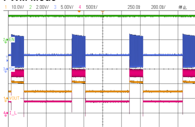
Figure 10.f V_{IN}=5\text{V} , V_{OUT}=12\text{V} , LOAD=400mA L=10\mu\text{H} , C_{OUT}=10\mu\text{F} , C_{IN}=4.7\mu\text{F}
